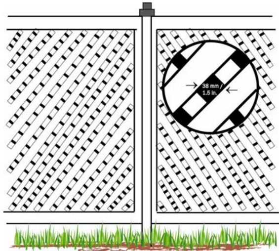
Recommended wood lattice opening
